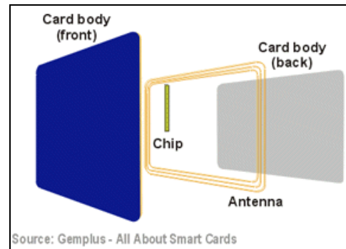
Gambar 6 Contactless Smart Card
