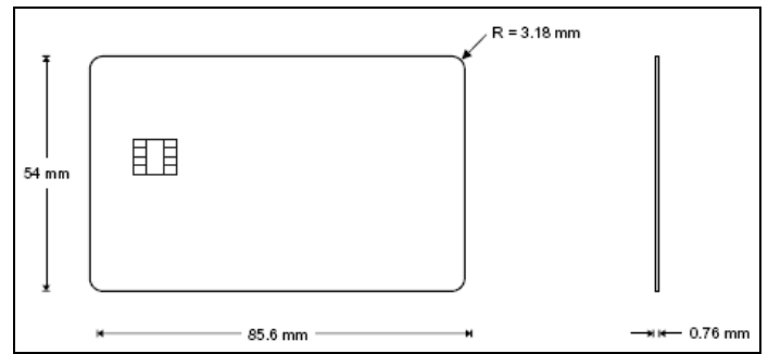
Gambar 2 Ukuran standar Smart Card format ID-1
