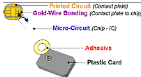
Gambar 1 Komponen Smart Card
