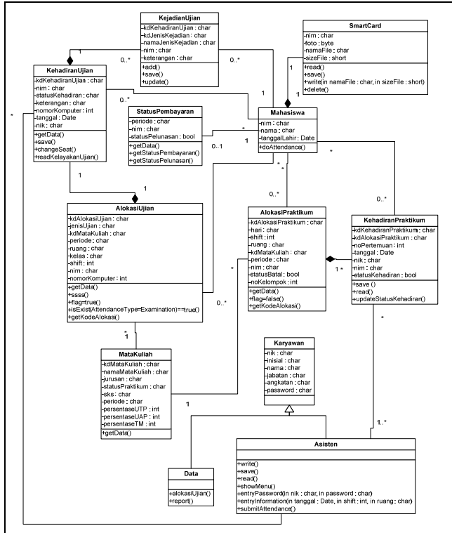
Gambar 12 Class Diagram
