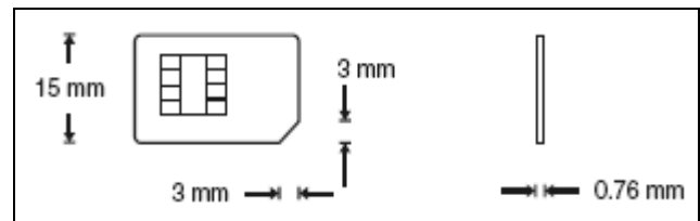
Gambar 3 Ukuran standar Smart Card format ID-000
